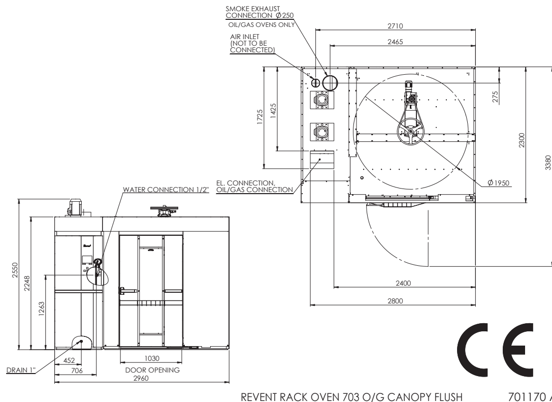
REVENT RACK OVEN 703 O/G CANOPY FLUSH
